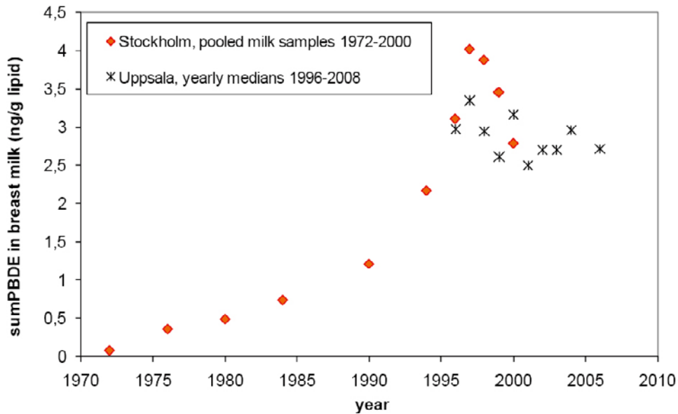
Figure 2.3.6.3-III: Levels of brominated flame retardants in breast milk samples (Livsmedelsverket 2011).
