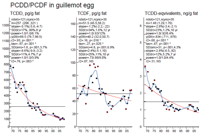
Figure 2.3.6.6-I: PCDD, PCDF (pg TCDD-eqv/g fat) and PCDD/F (ng TCDD-eqv/g fat) concentrations in guillemot eggs from Stora Karlsö (time series starting in 1970).
