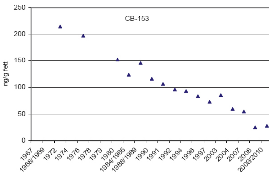
Figure 2.3.6.2-II: Levels of CB-153 in mother's milk in samples collected in Stockholm (Bergman et.al., 2010)
