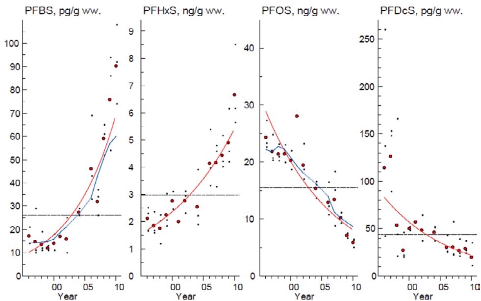
Figure 2.3.6.5-II: Concentrations of perfluorinated alkyl sulfonates in pooled samples (N=36) of blood serum from first-time mothers in Uppsala sampled between 1996 and 2010. The bigger red dots represents the geometric means for the pooled samples for each year. The red regression lines show significant linear trends for log-normal PFAS data. A running mean smoother (blue line) shows significant non-linear trend components. PFC's=perfluoroalkyl compounds, PFDcS=PFDS. (Glynn et al. (2011).
