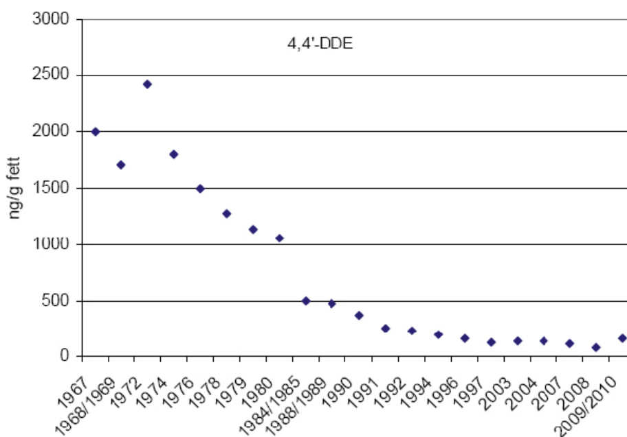
Figure 2.3.6.4-II: Levels of DDE in mother's milk in samples collected in Stockholm (Bergman et.al. 2010).
